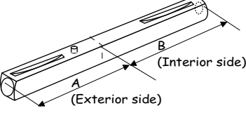
N7S-SCX Custom Straight Spindle
